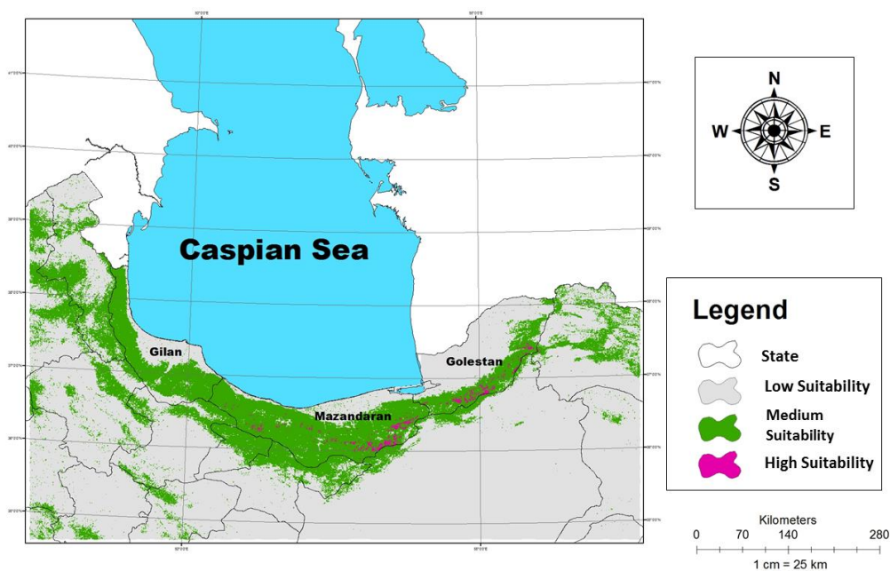
Figure 3. Suitability map of brown bear in the north of Iran
